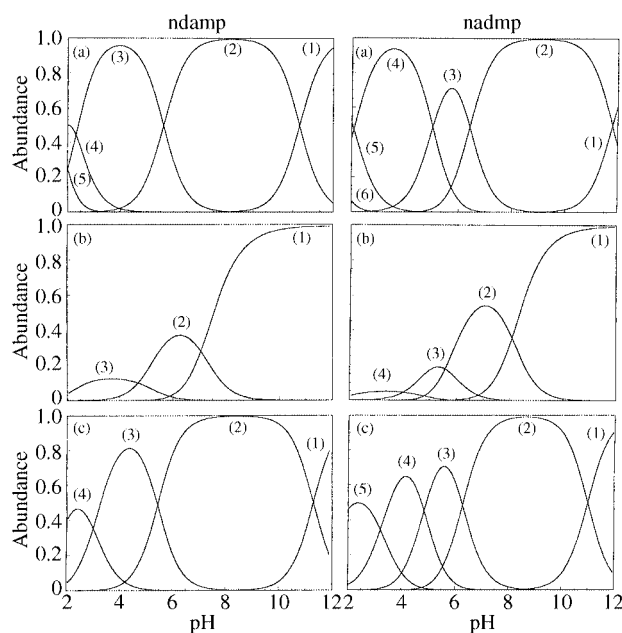
Fig. 1 Distribution diagrams: (a) ligand, (1) L, (2) HL, (3) H 2 L, (4) H 3 L, (5) H 4 L, (6) H 5 L, c_{\text{L}} = 0.01 mol dm −3 ; (b) strontium complex, (1) ML, (2) M(HL), (3) M(H 2 L), (4) M(H 3 L), c_{\text{L}} = c_{\text{Sr}} = 0.01 mol dm −3 ; (c) cadmium complex, (1) M(OH)L, (2) ML, (3) M(HL), (4) M(H 2 L), (5) M(H 3 L), c_{\text{L}} = c_{\text{Cd}} = 0.005 mol dm −3 .
