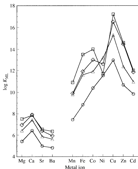
Fig. 2 Plots of the logarithmic formation constants of metal complexes. ○, nta; △, ndamp; ◇, nadmp; □, ntmp.
