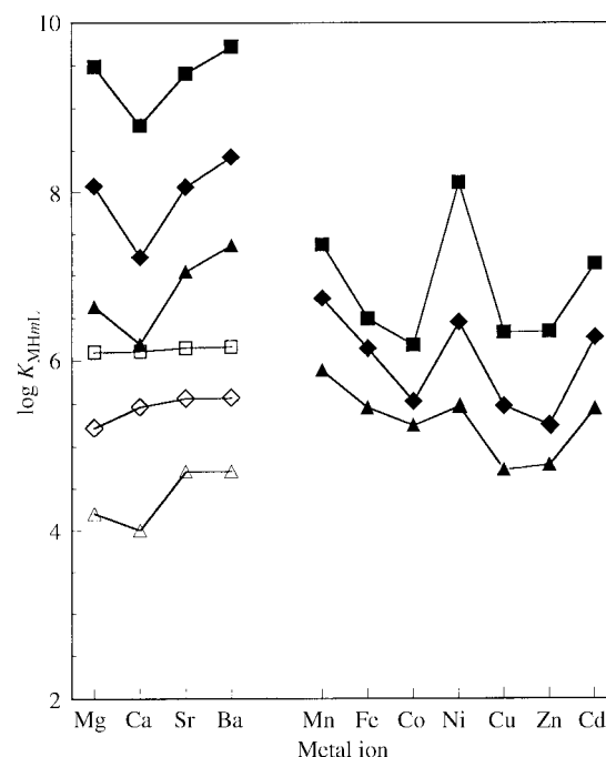
Fig. 3 Plots of the logarithmic protonation constants of metal complexes. ndamp: ▲, \log K_{\text{MHL}} ; △, \log K_{\text{MH}_2\text{L}} . nadmp: ◆, \log K_{\text{MHL}} ; ◇, \log K_{\text{MH}_2\text{L}} . ntmp: ■, \log K_{\text{MHL}} ; □, \log K_{\text{MH}_2\text{L}} .
